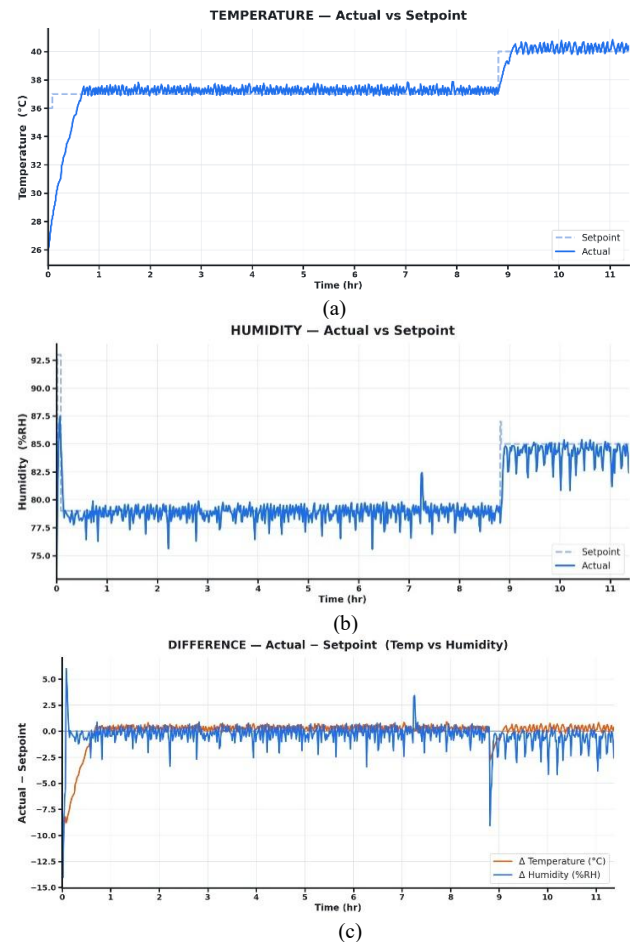
Fig. 18. Temperature and humidity profiles; (a) temperature, (b) humidity, and (c) difference between actual and setpoint.
