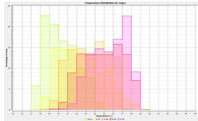
Fig. 7. Temperature distribution plot around the cages for different times
