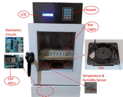
Fig. 17. Smart bee incubator build.
