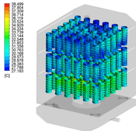
Fig. 8. Cage temperature at 220 seconds of operating first case.
